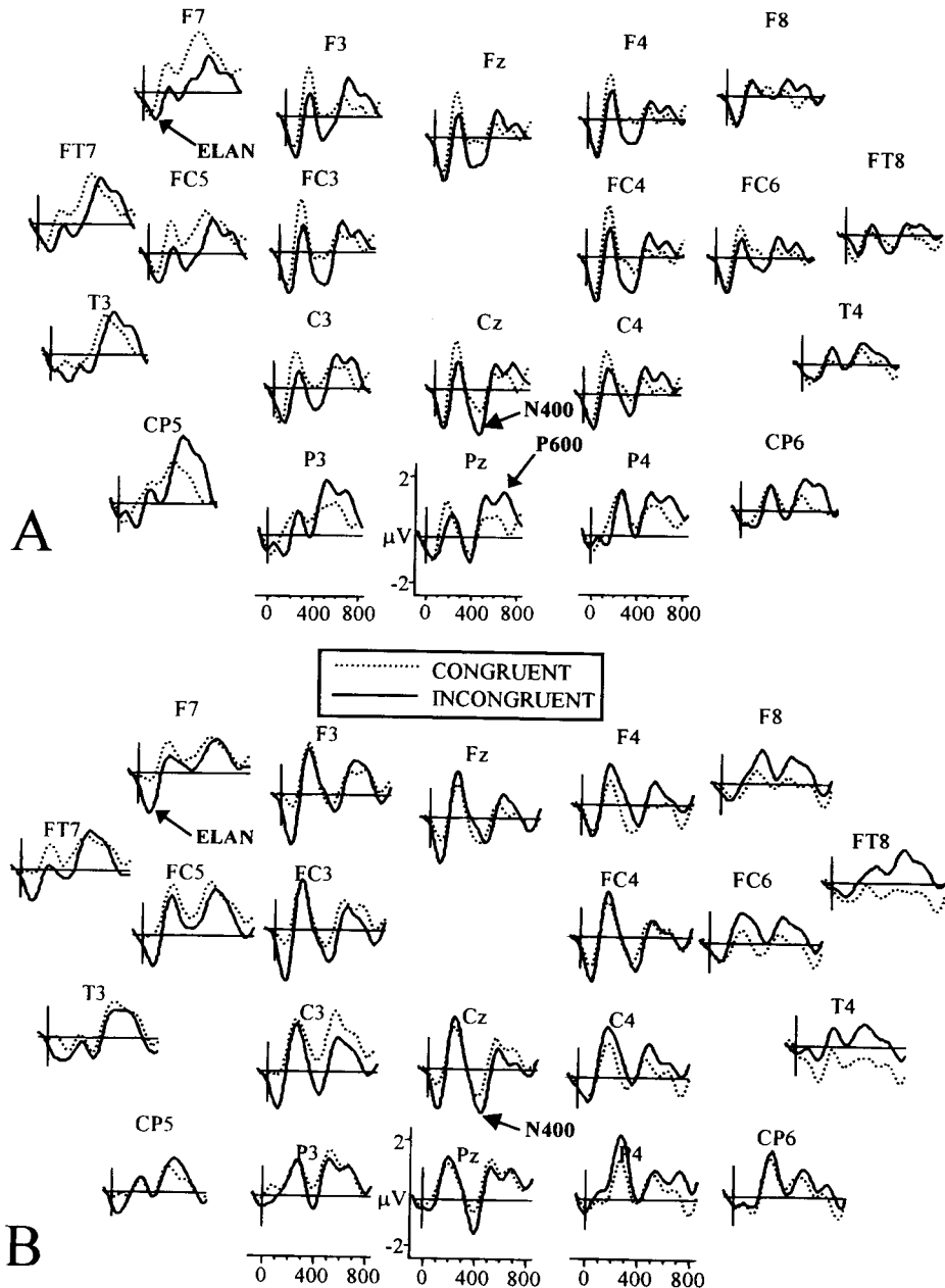
FIG. 3. The modulation of ERPs by syntactic congruity at selected channels for (A) marked predicates and (B) unmarked predicates. Note that the congruity effect on P600 is evident only for marked predicates and the N400 is modulated by congruity but not by markedness. The congruity effect on the early negativity (ELAN) is evident for both marked and unmarked predicates.
